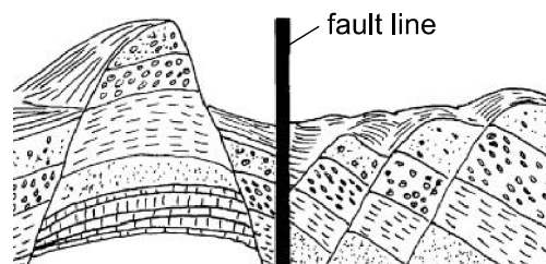
Fault-block mountains are formed by the movement of large amounts of rock along a crack in Earth's crust.
