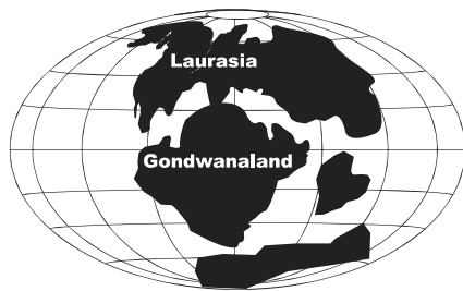
Laurasia and Gondwanaland
