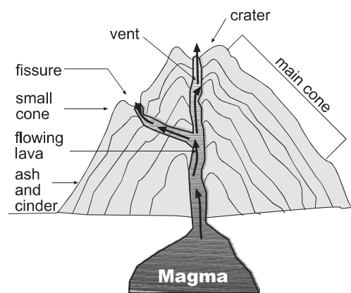
A volcano is an opening in Earth's surface through which melted rock, called magma, erupts from inside Earth.
