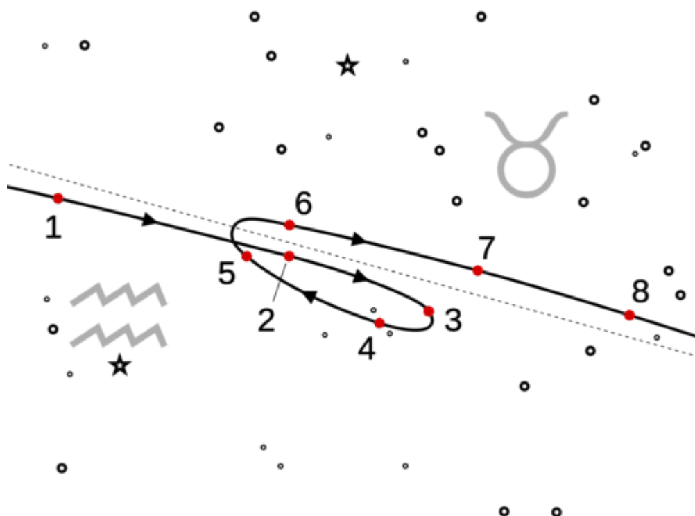
Retrograde motion of Mars as seen from Earth.
